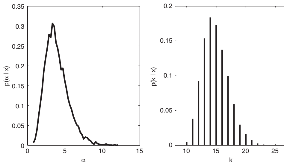
Fig. 15. Estimated posterior distributions over \alpha and k when the infinite groups model is applied to the publications data.
