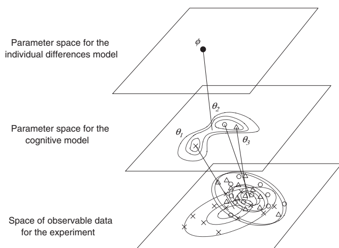
Fig. 2. The model-based view of individual differences. The data are plotted in the lower data space, with different symbols for each participant. The middle parameter space shows the parameter values inferred for each participant based on their data and an individual differences model that describes how these parameters can vary between people. The upper parameter space shows the inferred parameter values for this individual differences model.
