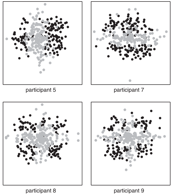
Fig. 14. Last 300 trials for subjects 5, 7, 8 and 9 in McKinley and Nosofsky’s (1995) experiment 2. Black dots denote “A” responses, and gray dots denote “B” responses.
