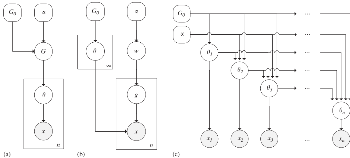
Fig. 4. Three graphical representations of a model employing a Dirichlet process prior. Each panel depicts the same model, but shown from a different perspective. Panel a depicts the standard view (Eq. (15)), panel b shows the Sethuraman construction (Eq. (16)) and panel c displays the construction via the Pólya urn scheme (Eq. (14)).
