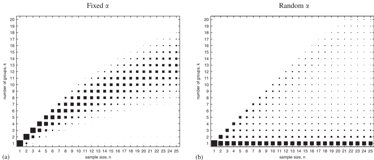
Fig. 8. Prior distributions over the number of components k for sample sizes n ranging from 1 to 25. The panel on the left shows the prior for a Dirichlet process with dispersion \alpha = 10 , where the area of each rectangle is proportional to the probability associated with the corresponding value of k for a given n . The panel on the right shows the marginal prior over k for a Dirichlet process mixture in which the prior over \alpha is an inverse Gamma( \cdot | 10^{-10} , 10^{-10} ) distribution.
