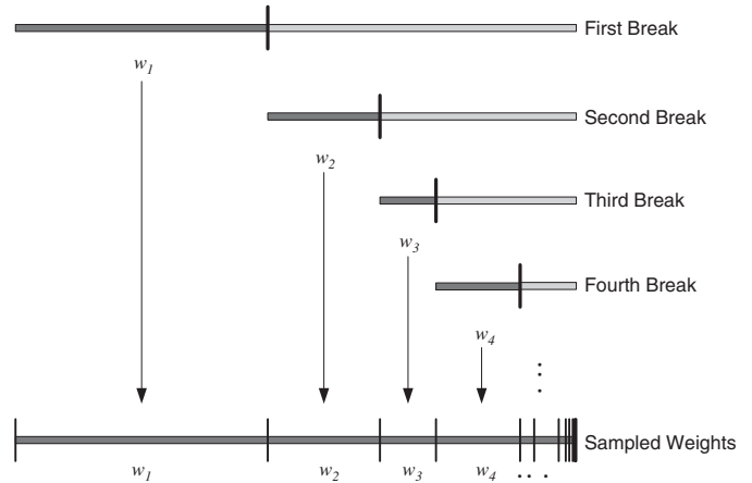
Fig. 5. A graphical depiction of the stick-breaking process, showing successive breaks of a stick with starting length one, and how the lengths of the pieces correspond to sampled weights.
