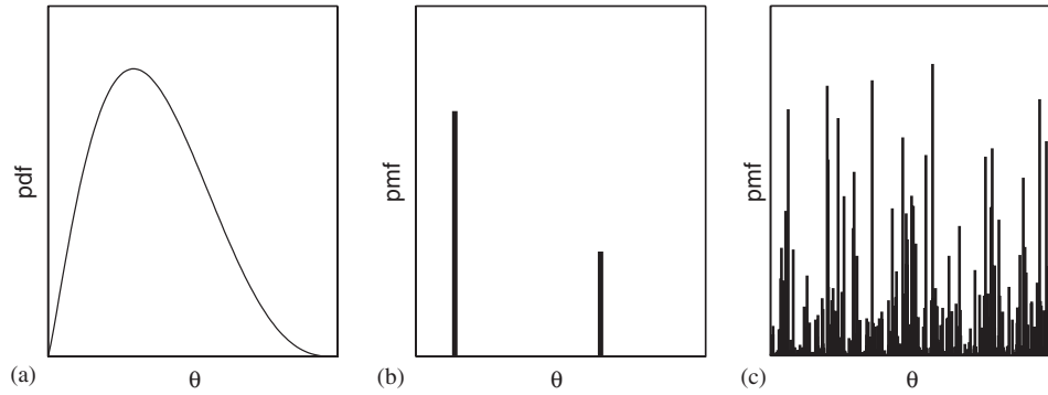
Fig. 3. Parameter distributions associated with stochastic parameters approach to individual differences (panel a), the original groups approach (panel b), and the infinite groups approach (panel c). The continuous measure shown in panel a is a probability density function (pdf) while the discrete measures in panels b and c are probability mass functions (pmf).
