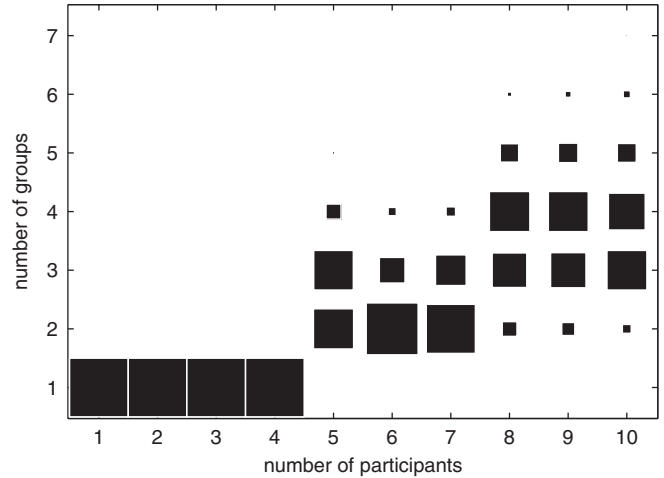
Fig. 12. Estimated posterior over k as a function of n . Assuming subjects arrive in a fixed order, from the first to the tenth person, we can see that the number of inferred groups changes as more people are observed. The area of the squares is proportional to the posterior probability of k given n .
