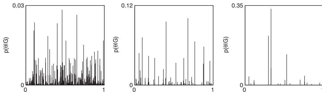
Fig. 7. Distributions sampled from a Dirichlet process with a uniform distribution over [0, 1] as the base distribution G_0(\cdot) , and dispersion parameters of \alpha = 100 (left), \alpha = 20 (middle), and \alpha = 5 (right). In all cases there are a countably infinite number of components (most of which are too small to see), but the distributions vary in the extent to which the probability mass is concentrated on a few points.
