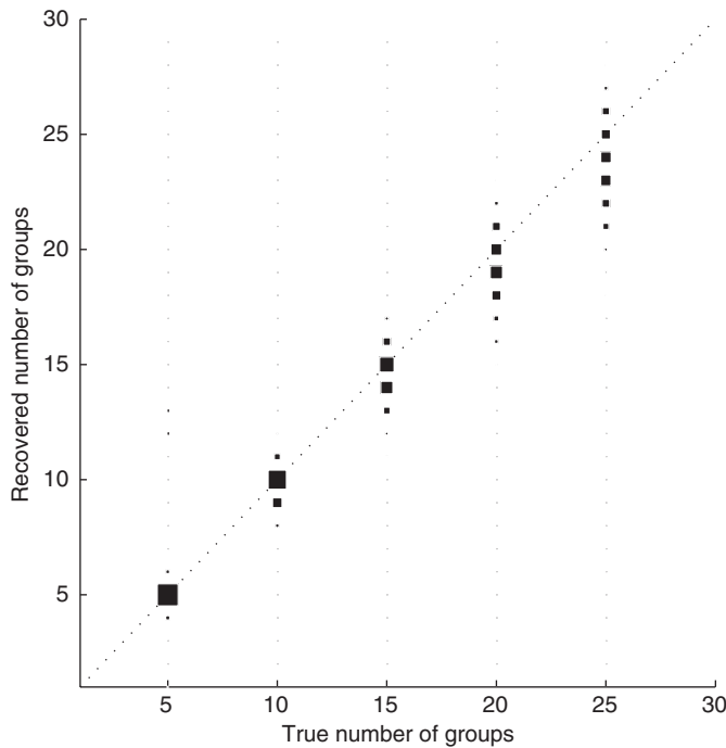
Fig. 10. Simulations in which n = 100 people provide s = 100 observations each, and m = 20 response options are possible on every trial. The true number of groups varies from 5 to 25. After a burn-in of only 500 samples, and using only a single draw from the posterior distribution, the Gibbs sampler performs reasonably well.
