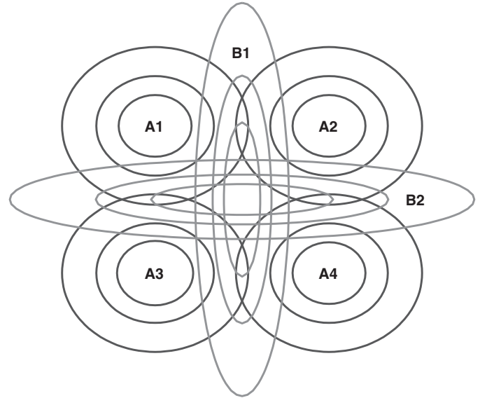
Fig. 11. The category densities used in McKinley and Nosofsky’s (1995) experiment 2. Category A (dark gray) is a mixture of four Gaussians, while category B (light gray) is a mixture of two Gaussians. The 30%, 60% and 90% confidence ellipses are shown for each of the six densities.
