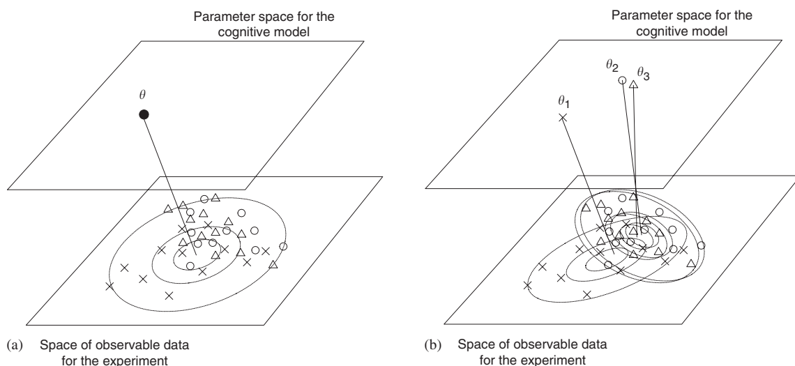
Fig. 1. Standard modeling approaches for data from many subjects, involving the aggregation of data (panel a), and the modeling of each individual independently (panel b). The data are plotted in the lower data space, with different symbols for each participant. The upper parameter space shows the parameter distributions inferred under each modeling approach.
